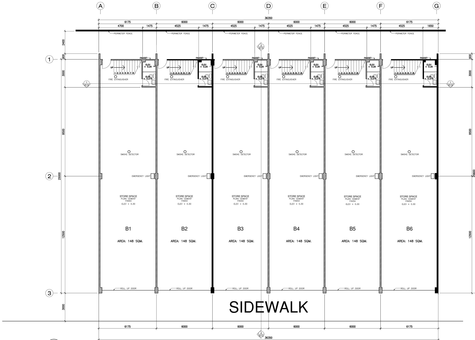
1 A8r GROUND FLOOR PLAN - BLDG B SCALE 1:100m
