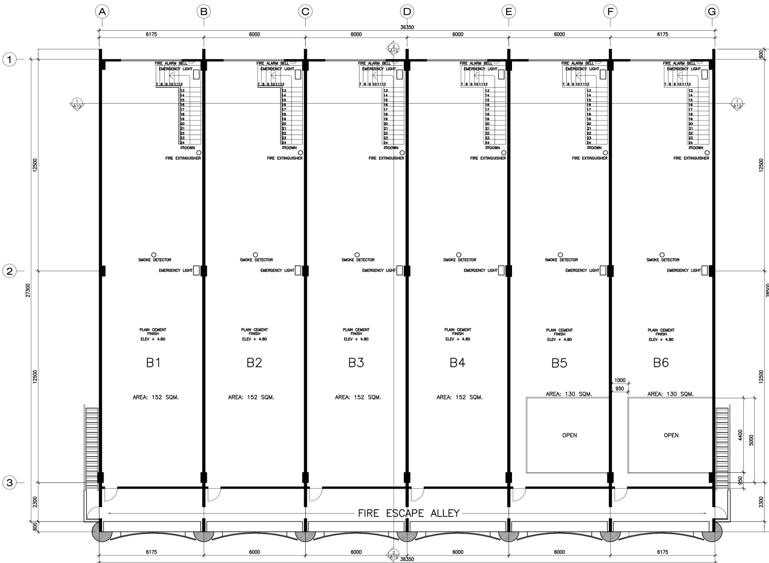
1 SECOND FLOOR PLAN - BLDG B A8r SCALE 1:100m
