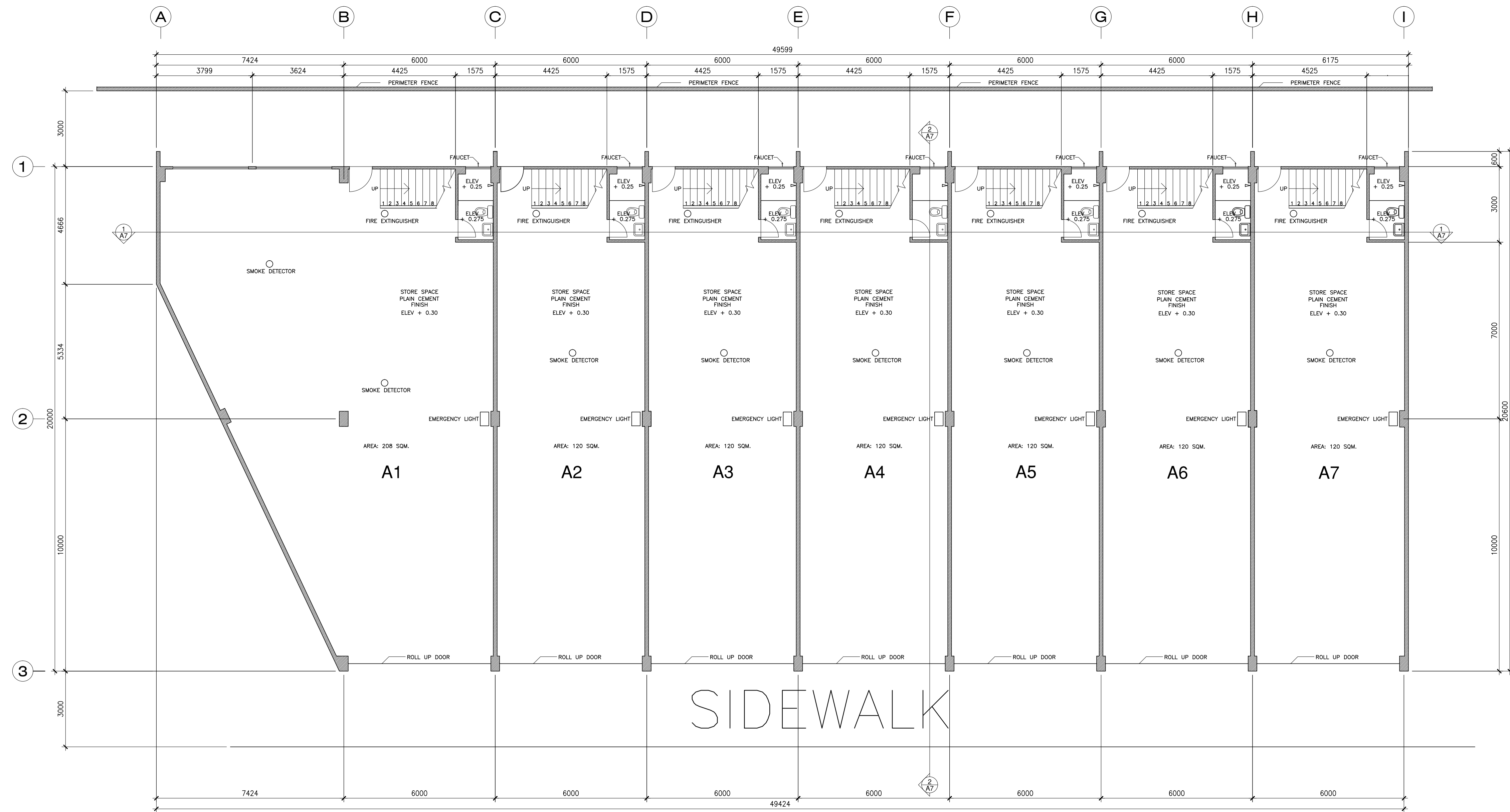
1 GROUND FLOOR PLAN - BLDG A A2r SCALE 1:100m
