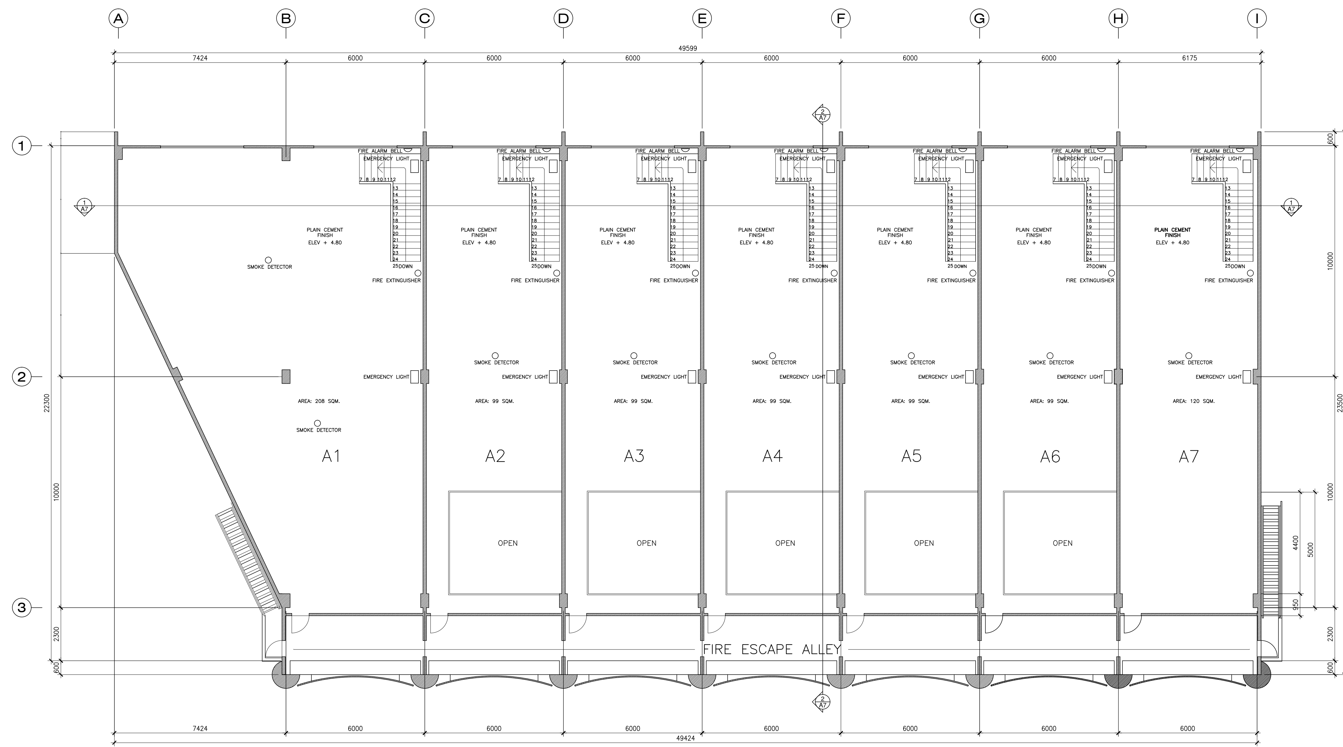
1 SECOND FLOOR PLAN - BLDG A A3r SCALE 1:100m
